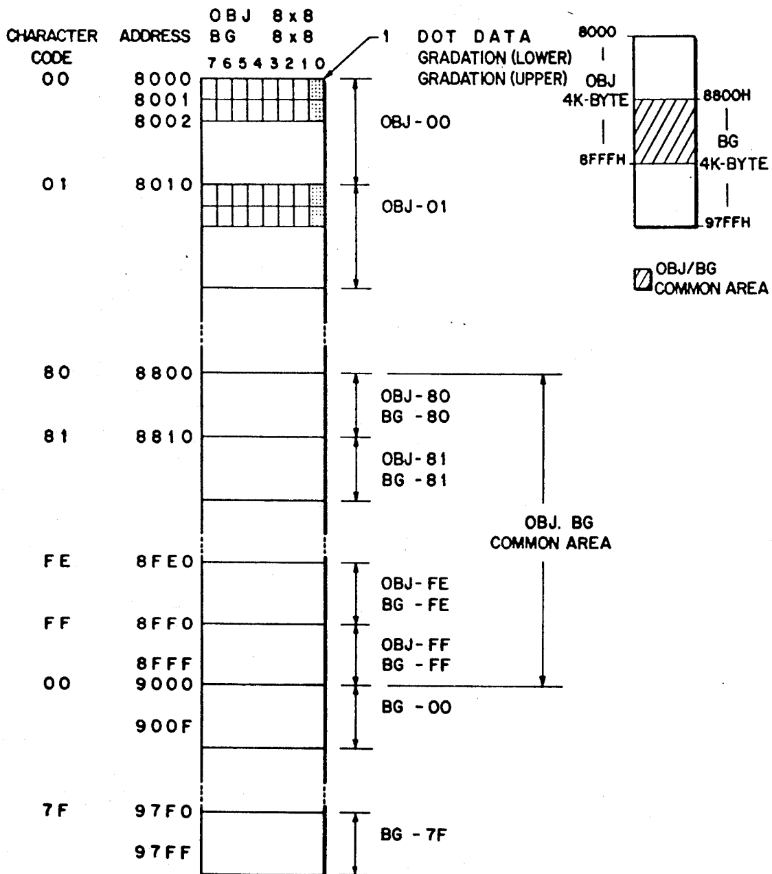
FIG. 13 CHARACTER RAM
